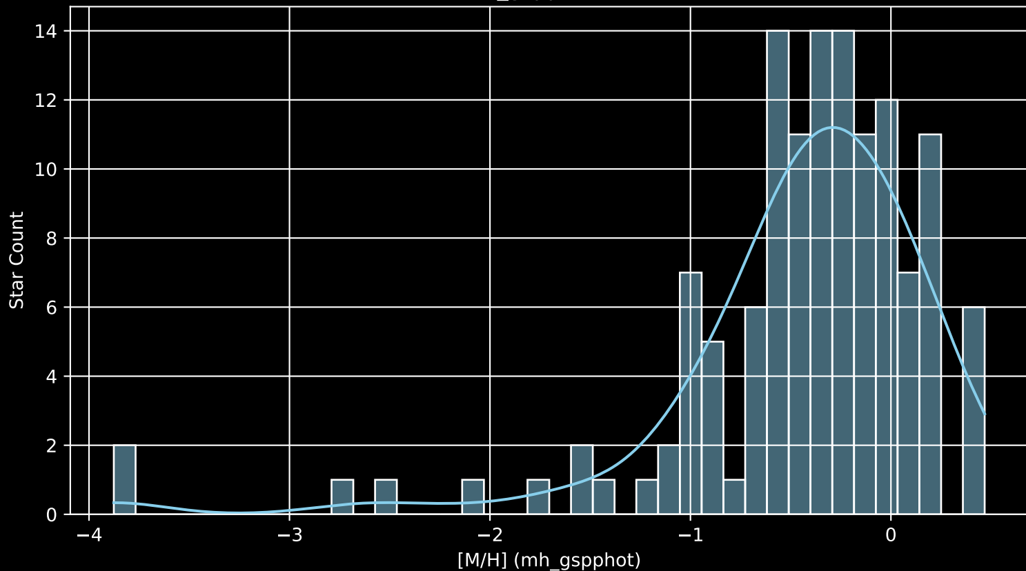
APOGEE DR17 Field: [352+18-O [M/H] (mh_gspphot) (n= 131)
