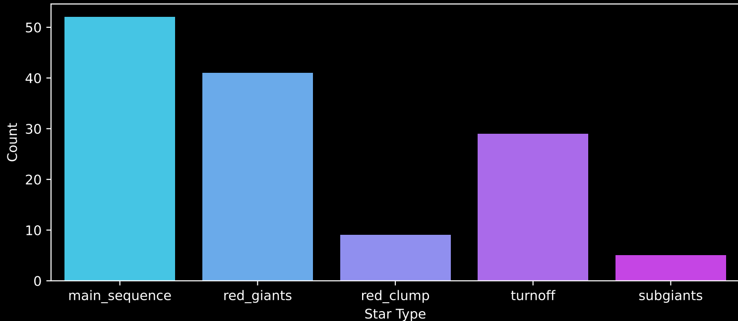
APOGEE DR17 Field: [352+18-O] Count plot of Star Type
