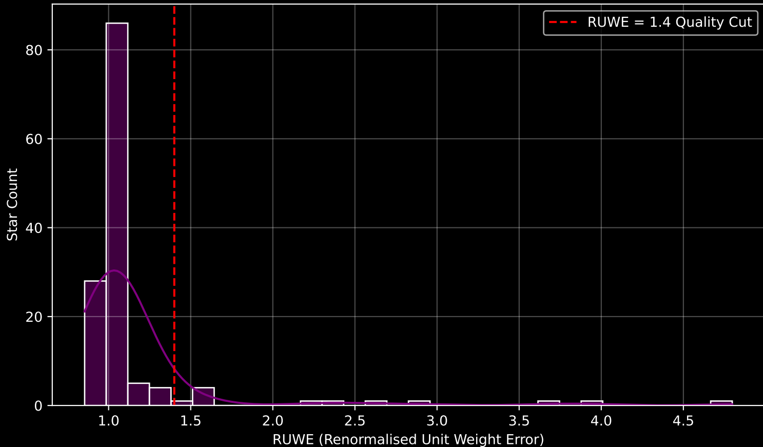
GAPOGEE DR17 Field [352+18-O] RUWE Distribution (n= 135)
