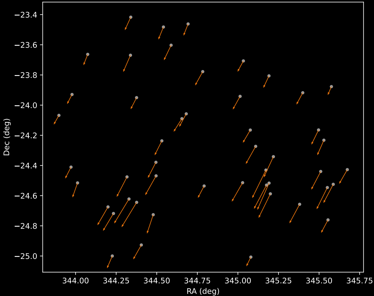
APOGEE DR17 Cluster 2 Proper Motion Vectors (n=48)
