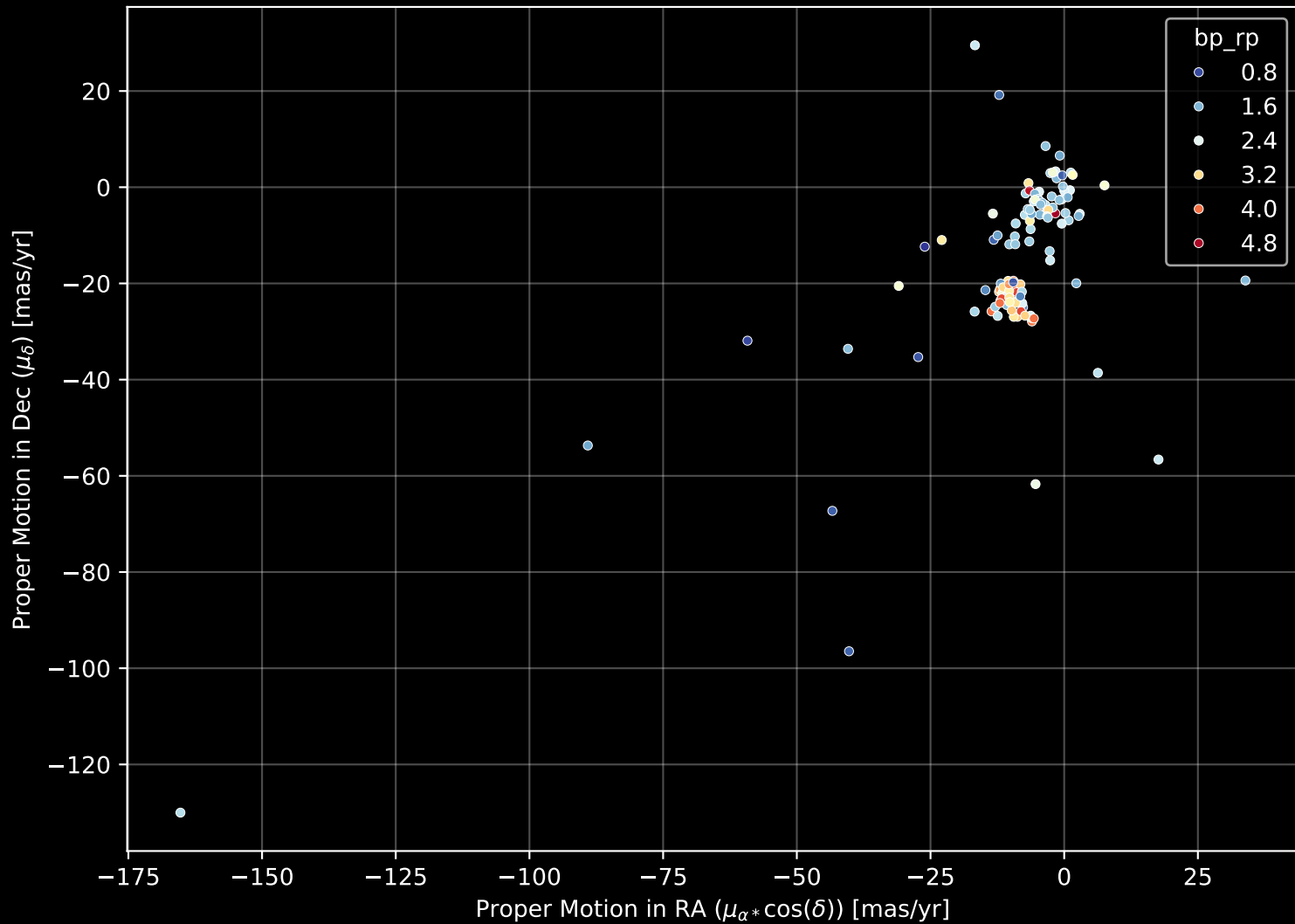
APOGEE DR17 Field: [352+18-O] Proper Motion Diagram (n= 136)
