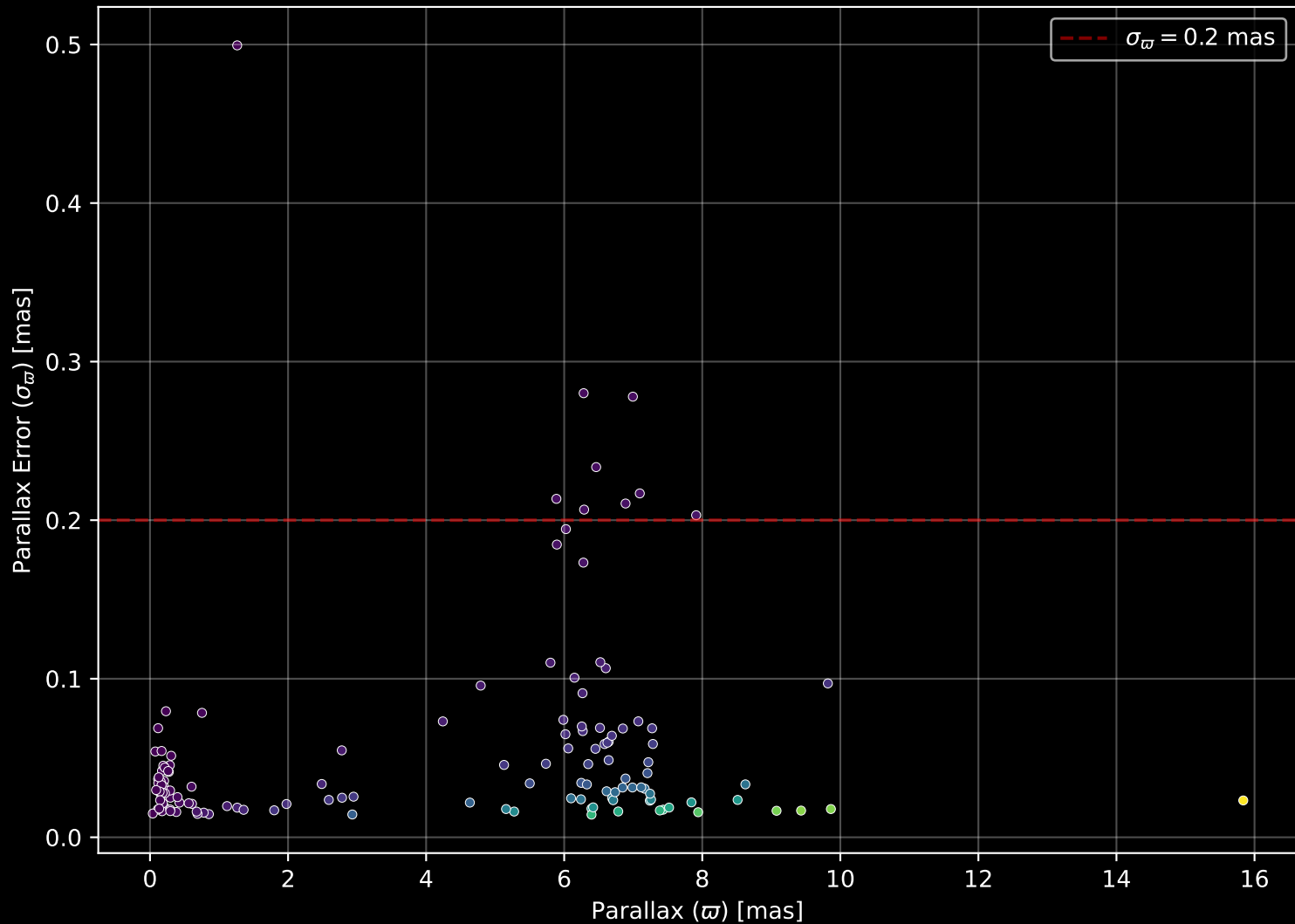
APOGEE DR17 Field: [352+18-O] Parallax Quality (n= 136)
