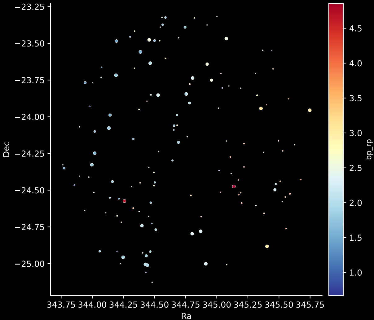
APOGEE DR17 Field: [352+18-O] Stars: 136
