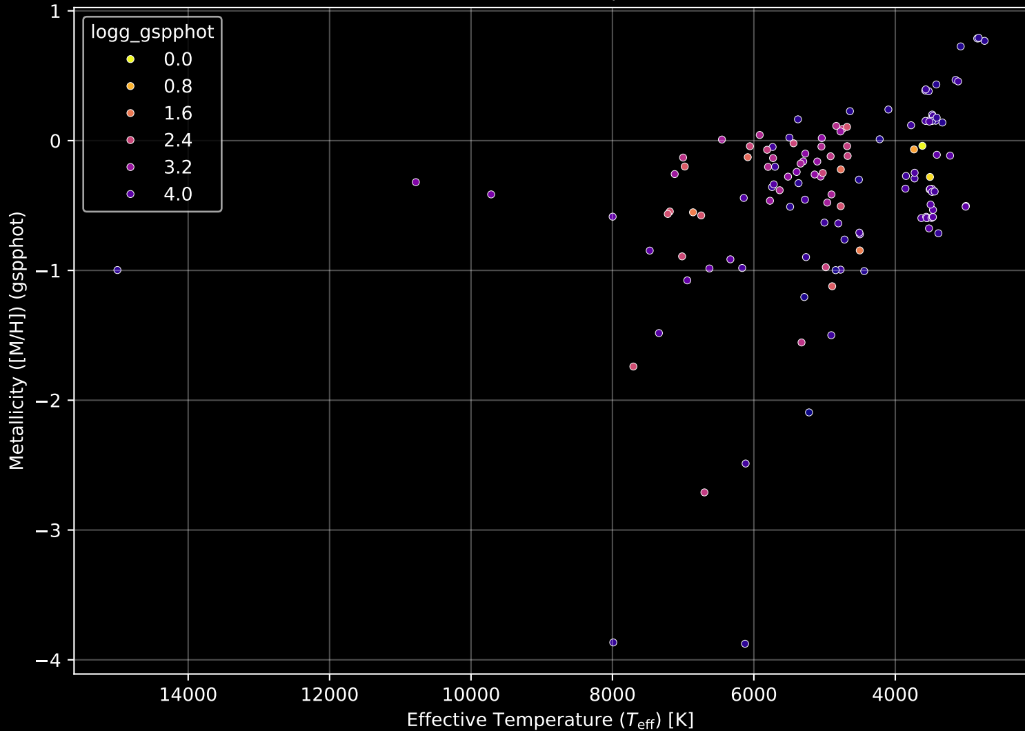
APOGEE DR17 Field: [352+18-O] Stellar Population Parameters (n= 136)
